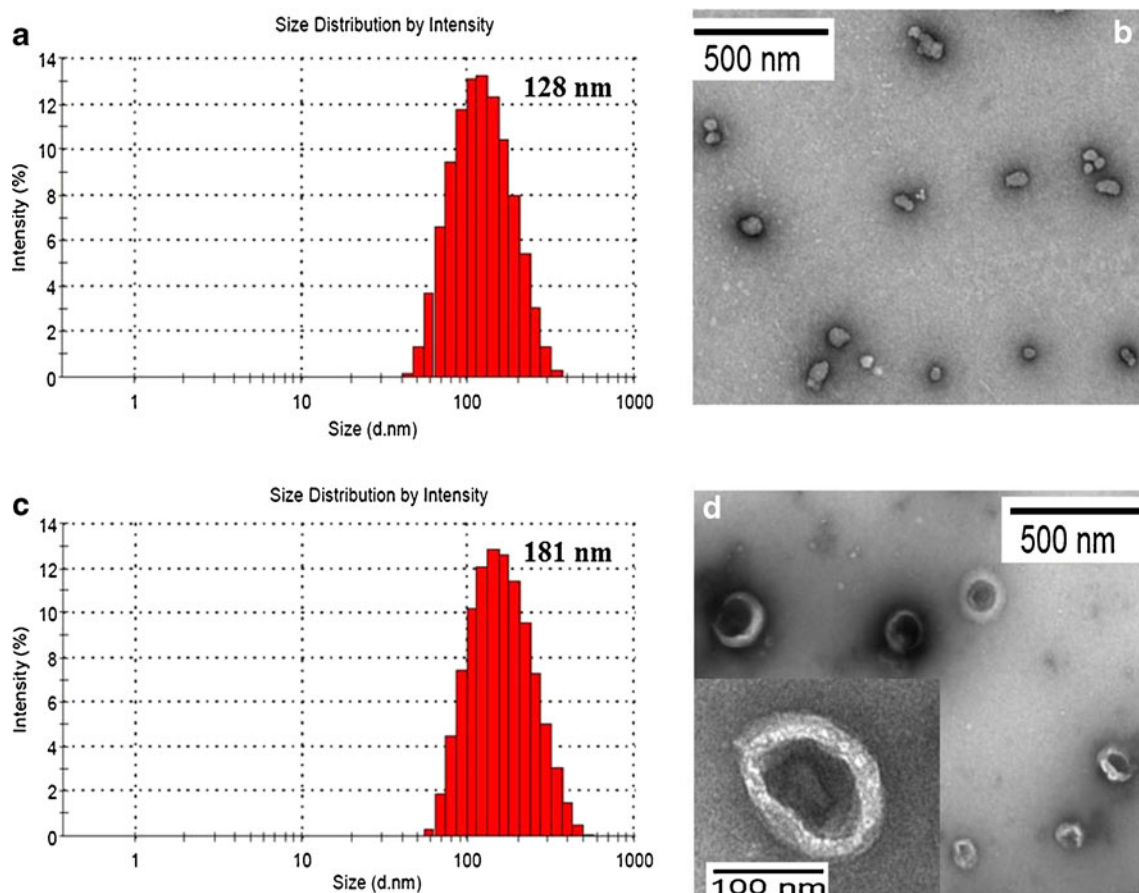
Fig. 2 Particle size and morphology of nanoparticles: (a) Dynamic light scattering (DLS) size measurement of FL-ceramide and TR-ceramide co-loaded liposomes; (b) TEM image of PLGA nanoparticles; (c) DLS size measurement and (d) TEM image of FL-ceramide and TR-ceramide co-loaded PLGA/liposome hybrids.
